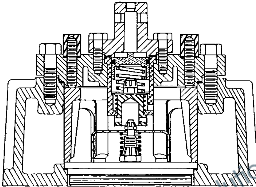
ASSEMBLY SUCTION
